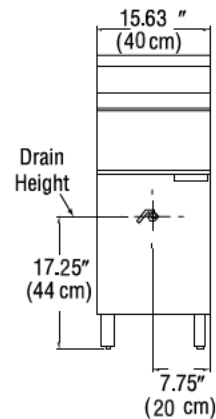
Front View
