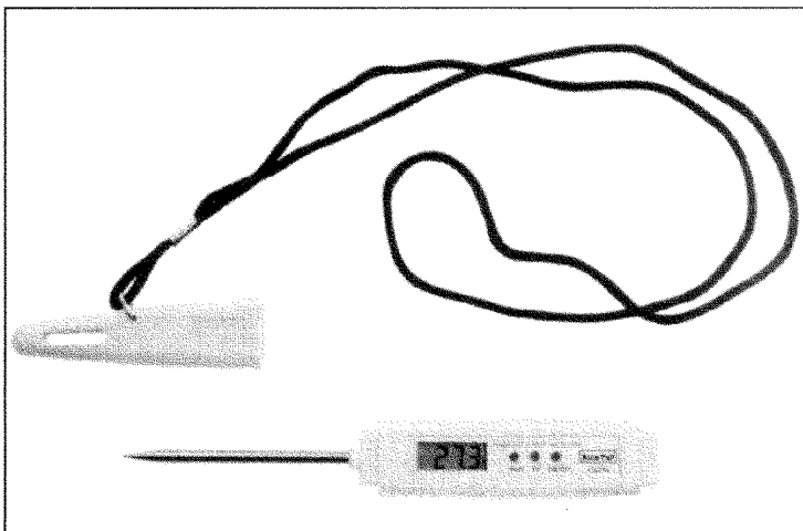
12710 Thermometer Shown with Removable Protective Cap and Neck Lanyard
