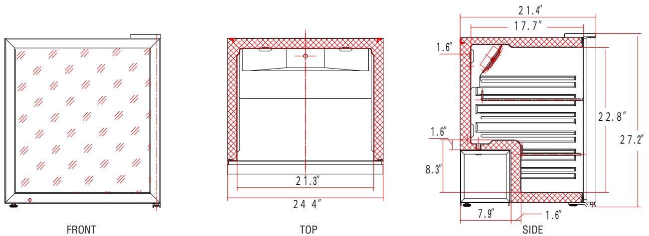
HUBM-3.5RB / HUBM-3.5FB
