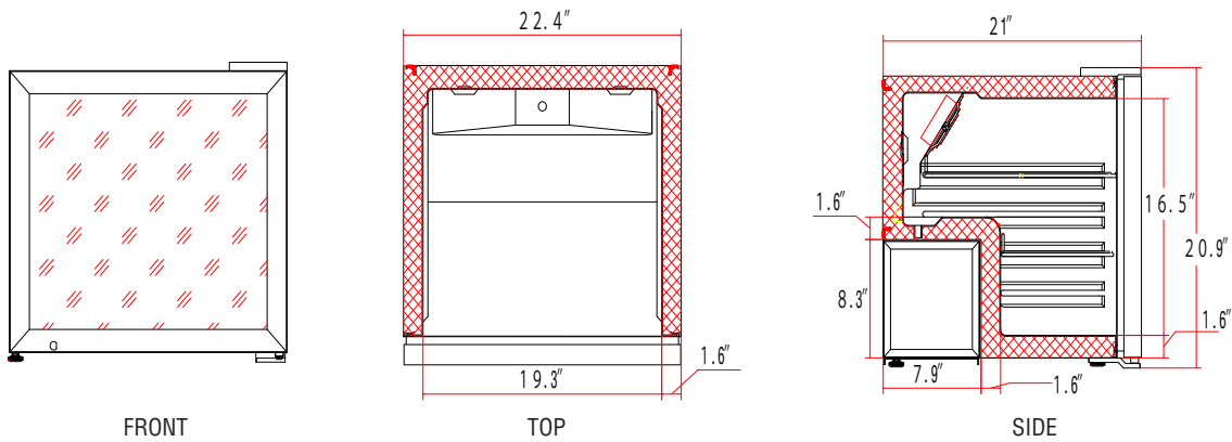
HUBM-2RB / HUBM-2FB
