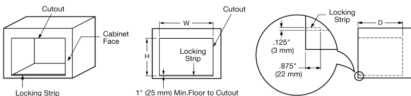
Locking Strip position for cut-out requirements
