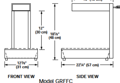
Model GRFFC
