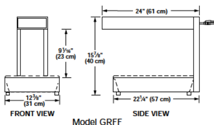
Model GRFF
