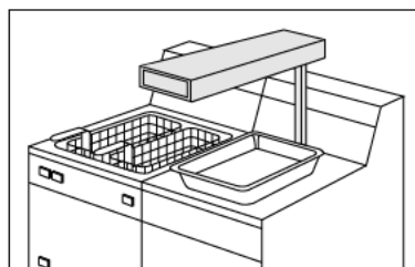
Model GRFS, GRFSL, GRFSC, GRFSCCL with swing-away post mount and cord with plug.
