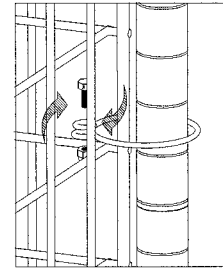
STEP 4 Secure loop on inside of cage
