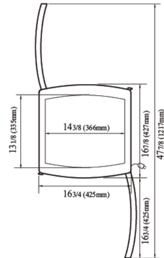
PLAN VIEW
