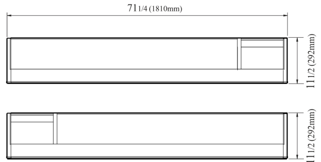
SAKURA-70R / SAKURA-70L FRONT VIEW
