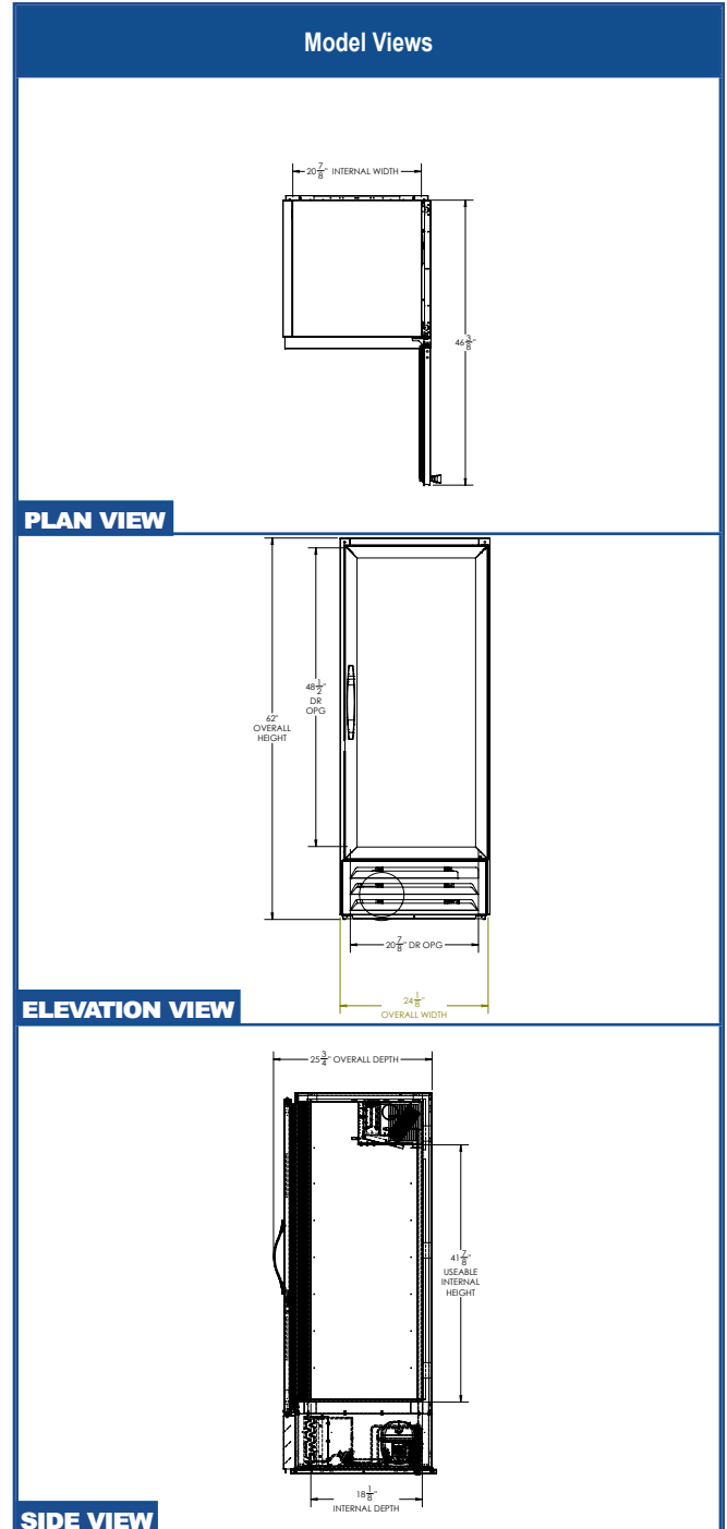
SIDE VIEW
