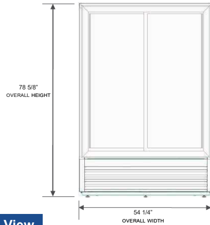
Elevation View
