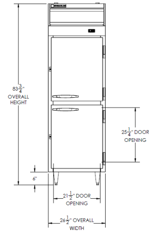
Elevation View
