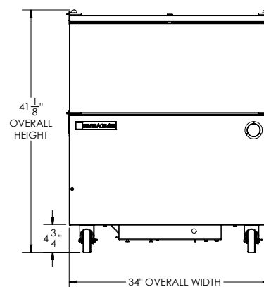
ELEVATION VIEW
