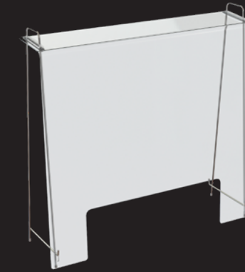
EB 738 E 001 Barrier with pass-through window 35.43" L x 9.84" D x 34.06" H, 10.14 lbs 1 ea
