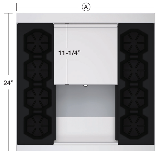
TOP VIEW OF KR24 ICE BIN WITH PARTIAL SLIDING COVER OPEN
