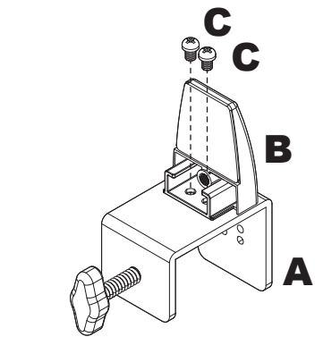
① Attach B to A with Screws C
